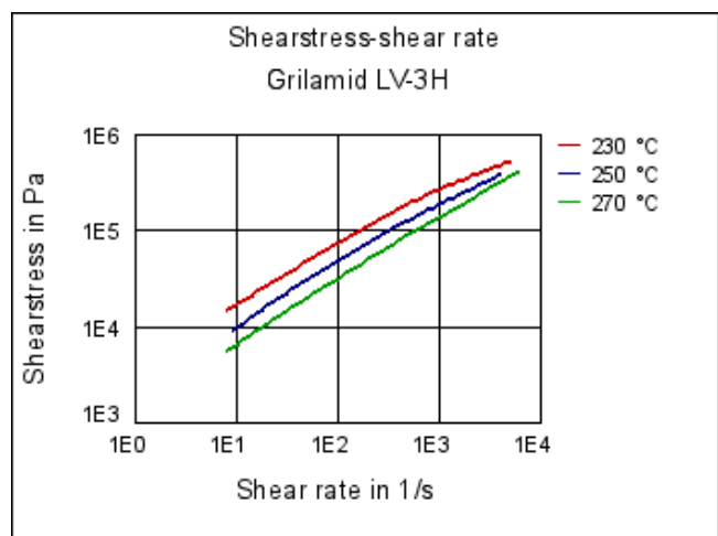
Shearstress-shear rate
