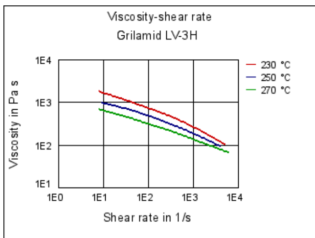
Viscosity-shear rate
